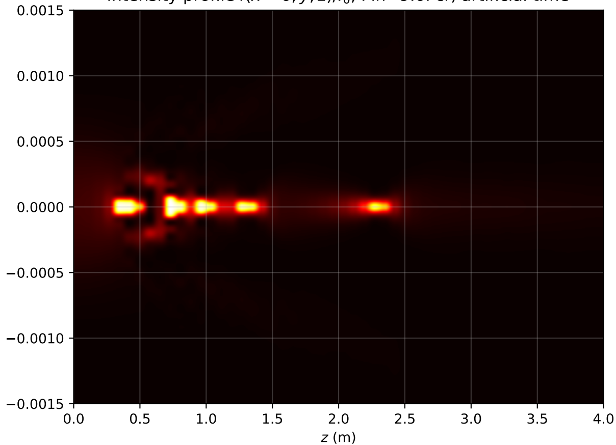
Intensity profile I(x = 0, y, z)/I_0 , P_{in}=9.0P_{cr} , artificial time
